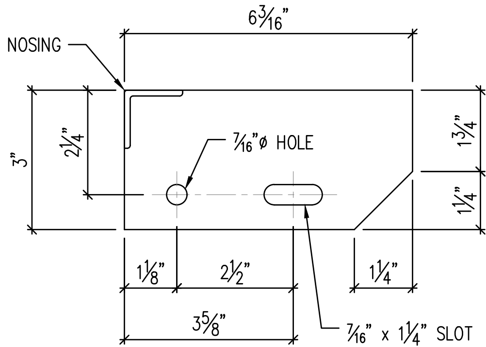
3" x 3/16" ALUMINUM END PLATE FOR 6 3/16" STAIR TREADS
