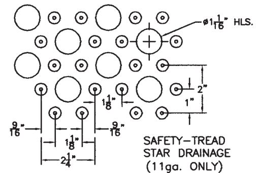
SAFETY-TREAD STAR
