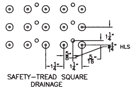
SAFETY-TREAD SQUARE
