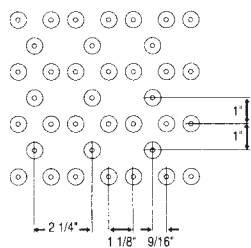
Safety-Tread® Star
